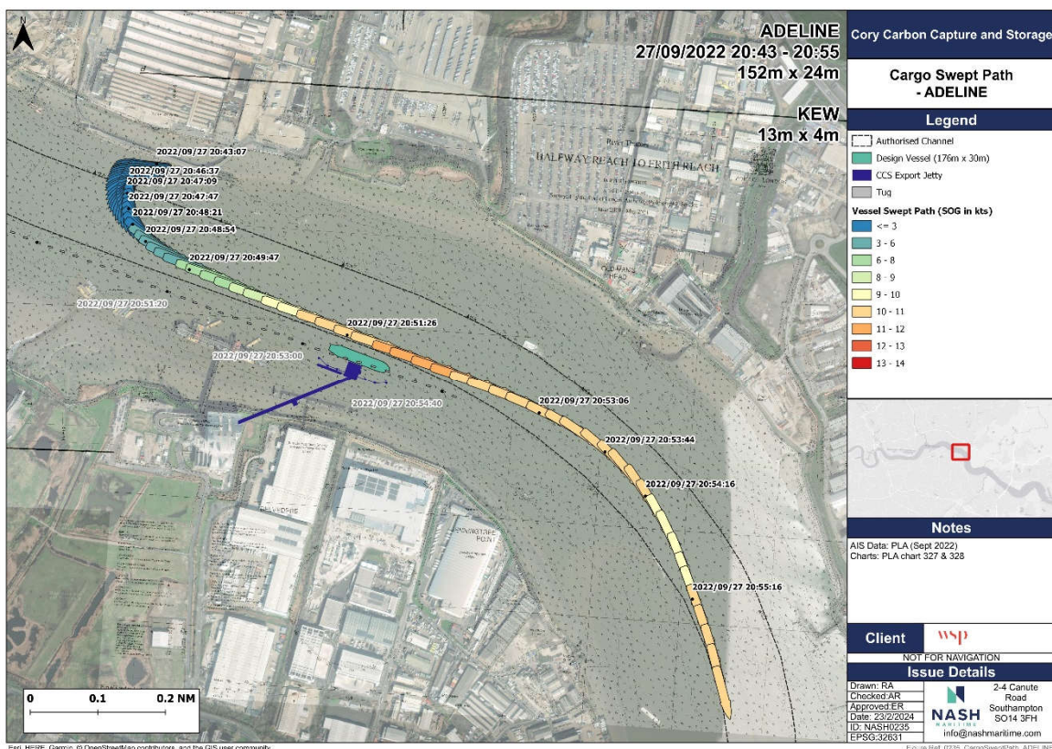
Figure 27: Swept path Ford's Jetty Departure (Adeline)
