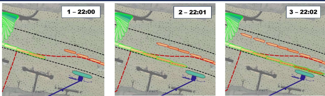
Figure 47: Swept path analysis showing the dredger Hanson Thames and the cargo vessel Wilhelmine on 30-Oct-23 at approximately 22hr00
